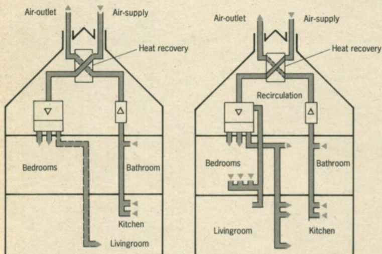
Two balanced ventilation systems.
